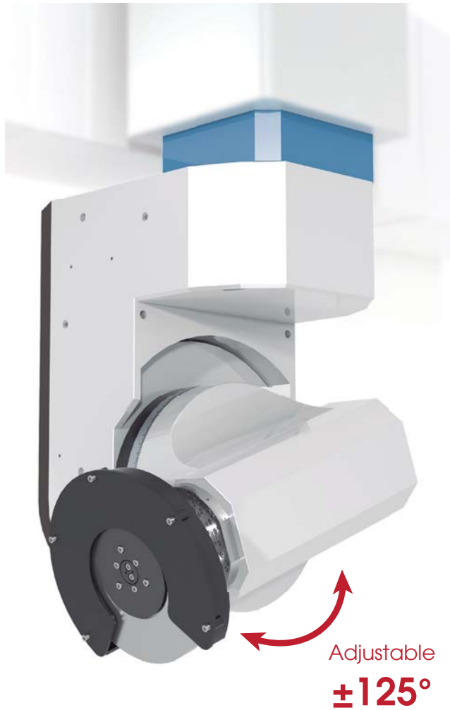
G.129 Coaxial with RAM Axis with Electrospindle
